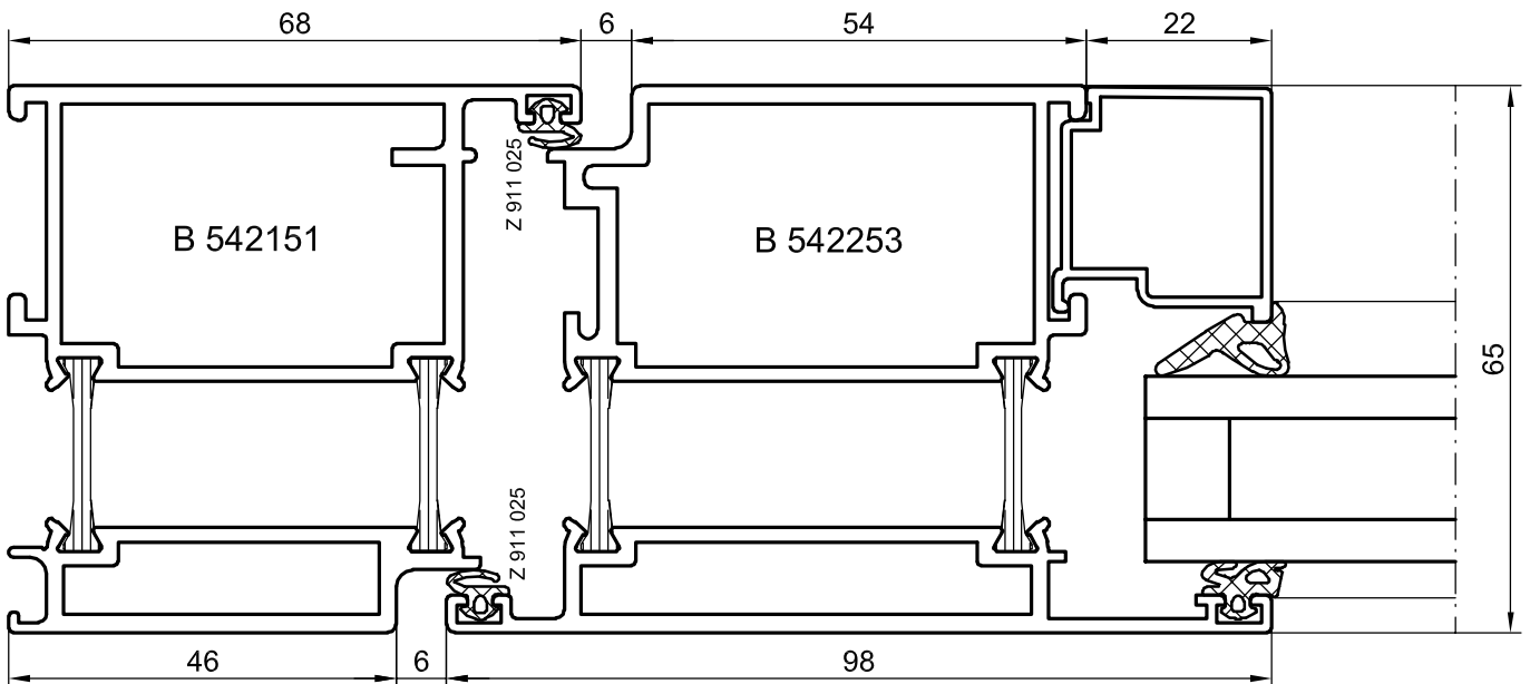
Horizontal section - opening out
