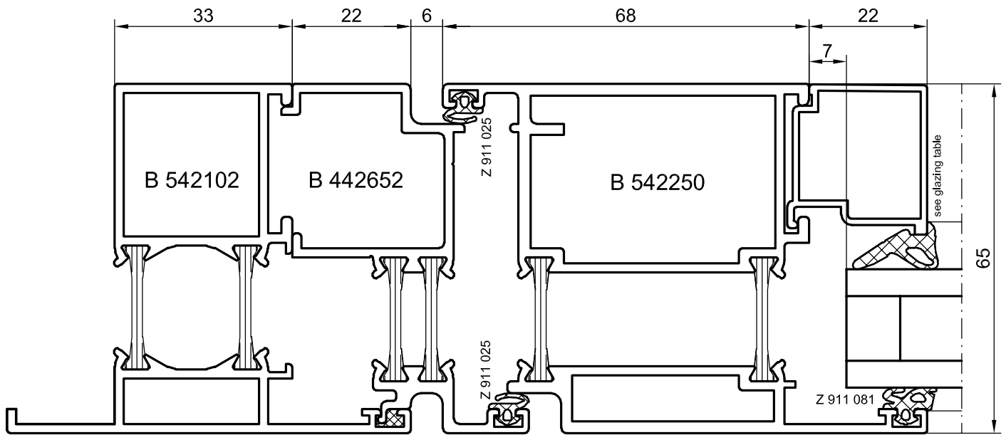
Horizontal section with supplementary profile - opening in
