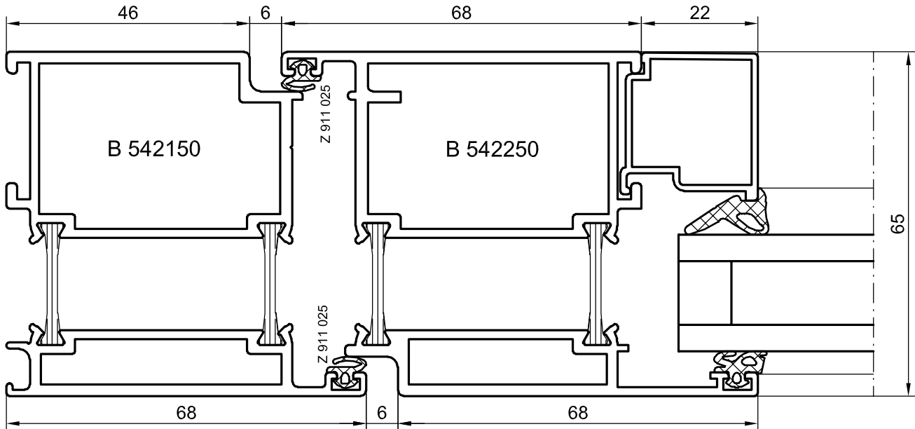
Horizontal section - opening in
