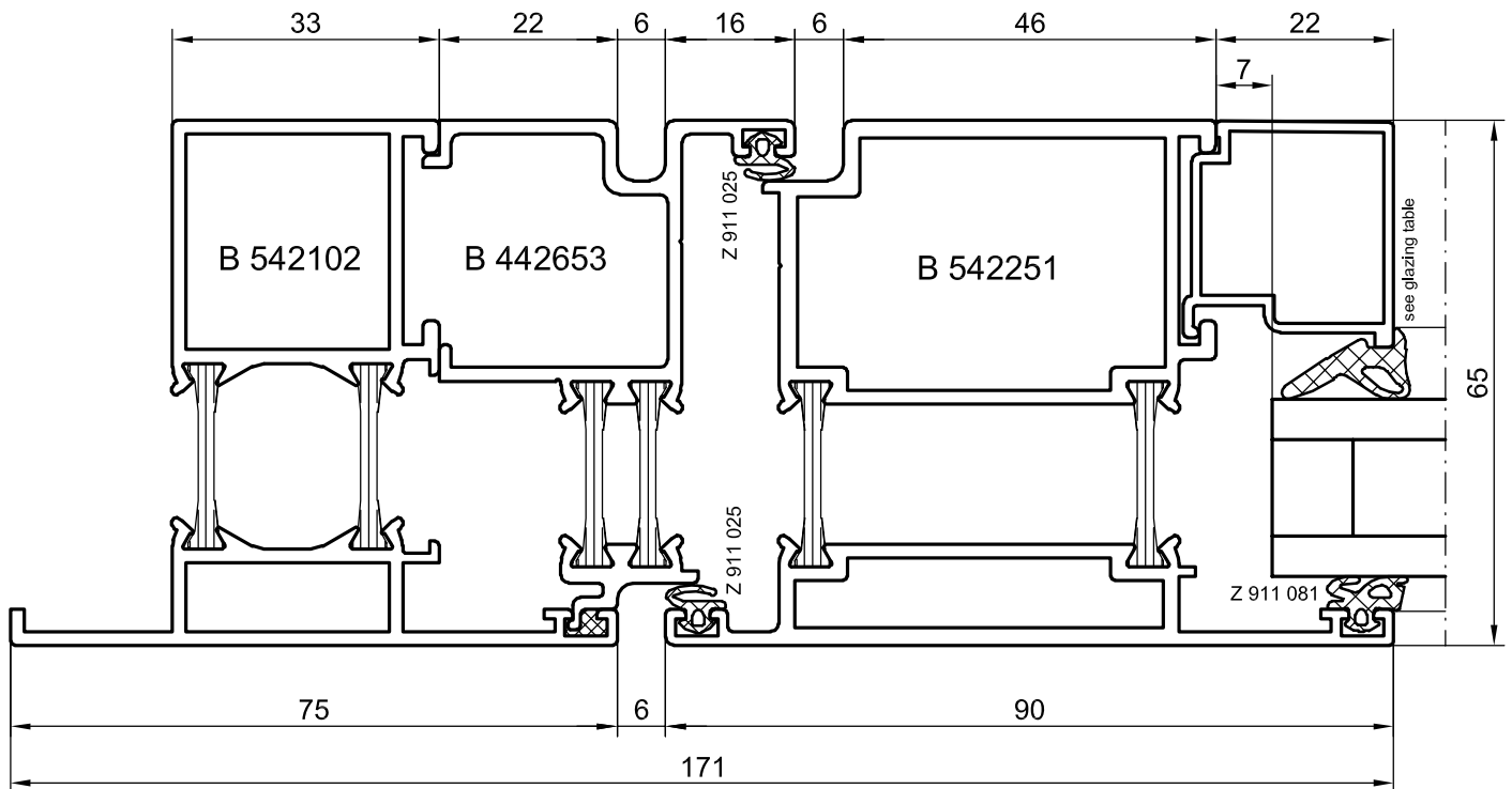
Horizontal section with supplementary profile - opening out
