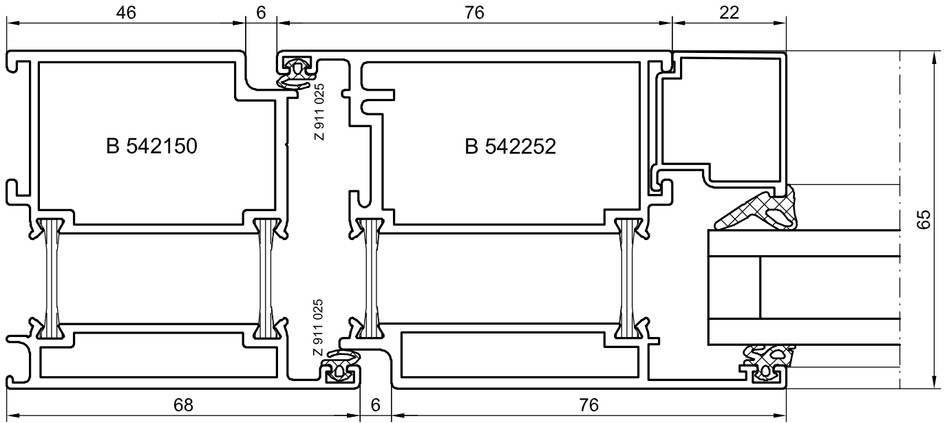
Horizontal section - opening in
