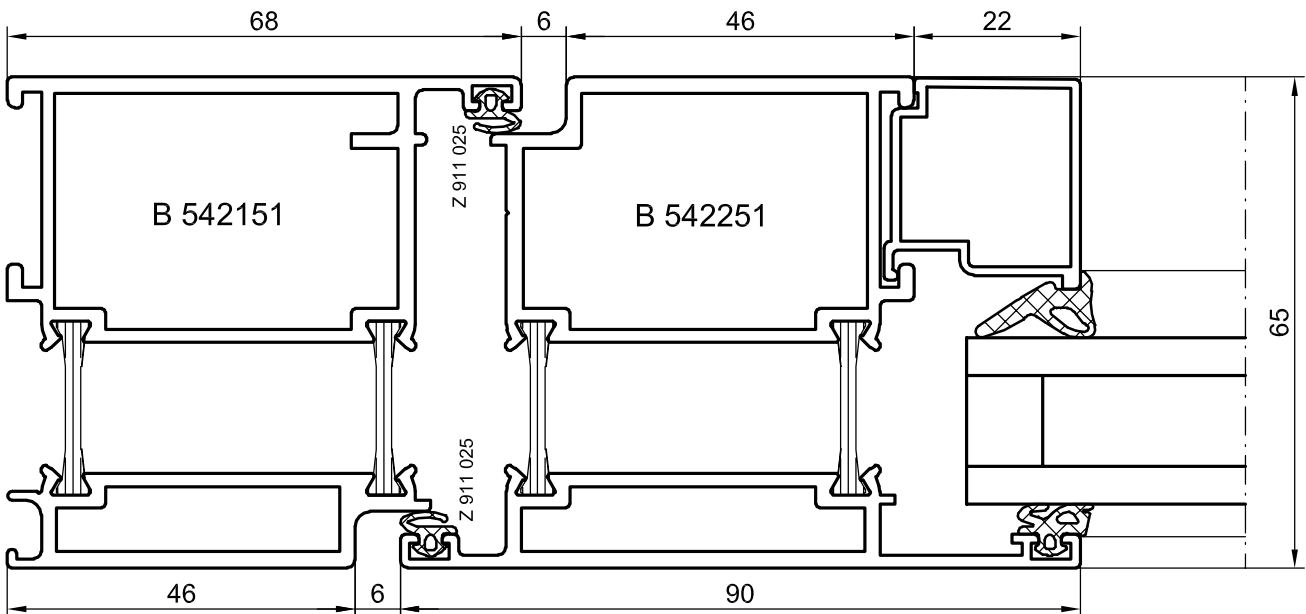
Horizontal section - opening out
