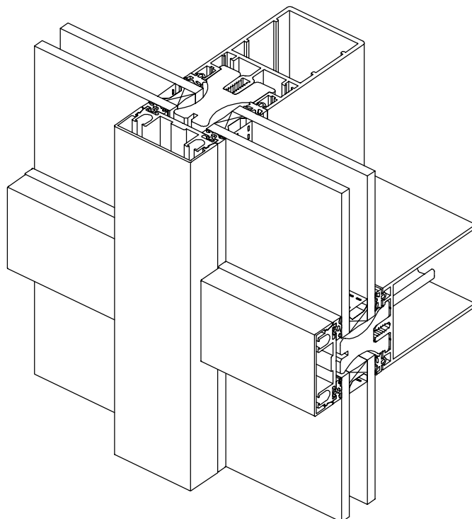
System: Deepened transom with insulating profile
