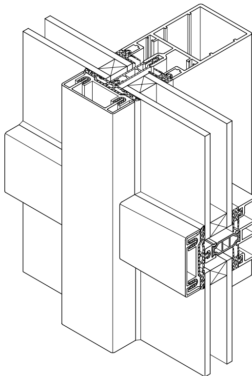
System: Inlet transom
