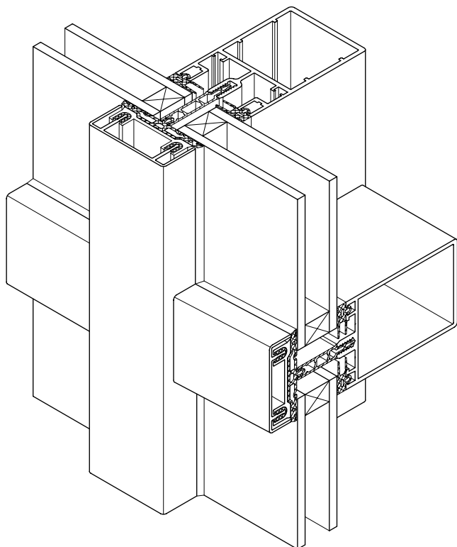
System: Deepened transom with spacer profile
